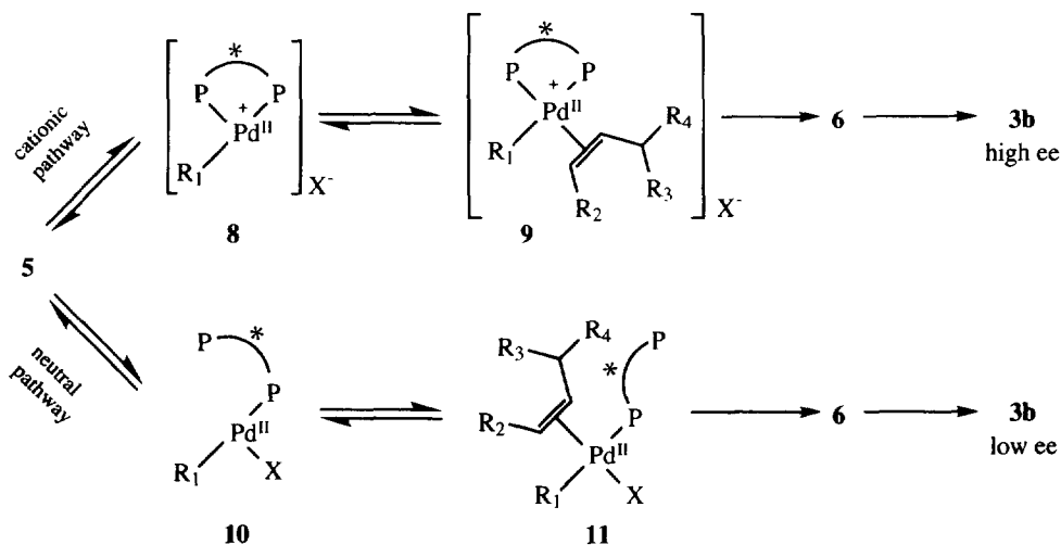
Scheme 2. Cationic and neutral pathways for the AHR mechanism.
